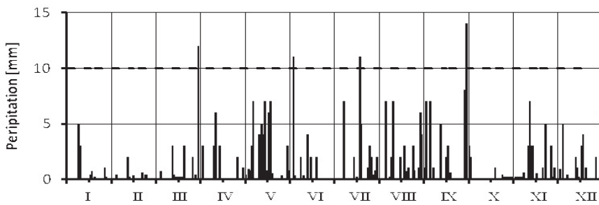
Fig. 5. Daily precipitation in 2010 at weather station Wrocław Port Lotniczy
