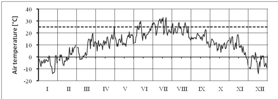
Fig. 4. Air temperature at 12.00 p.m. in 2010 at weather station Wrocław Port Lotniczy
