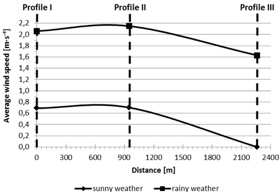
Figure 2. Changes in wind speed as the wind progresses along the flow path
