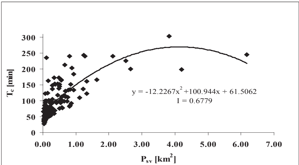
Figure 8. Dependence of the concentration time on the slope area [Mašíček, 2010a]
