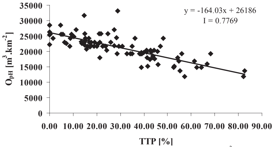
Figure 7. Dependence of the direct runoff volume from an area of 1 km 2 on grasslands (TTP) [Mašíček, 2010a]
