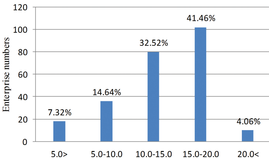
Figure 7. Ratio of ventilation opening to floor area
