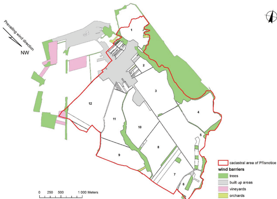
Figure 4. Wind barriers inside and outside (but in the prevailing wind direction) of cadastral area of Přisnotice
