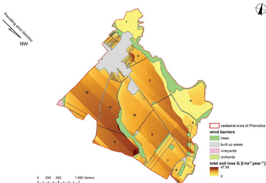
Figure 5. Wind erosion intensity in the cadastral area of Přisnotice in various distances from barriers (without their protective effect)
