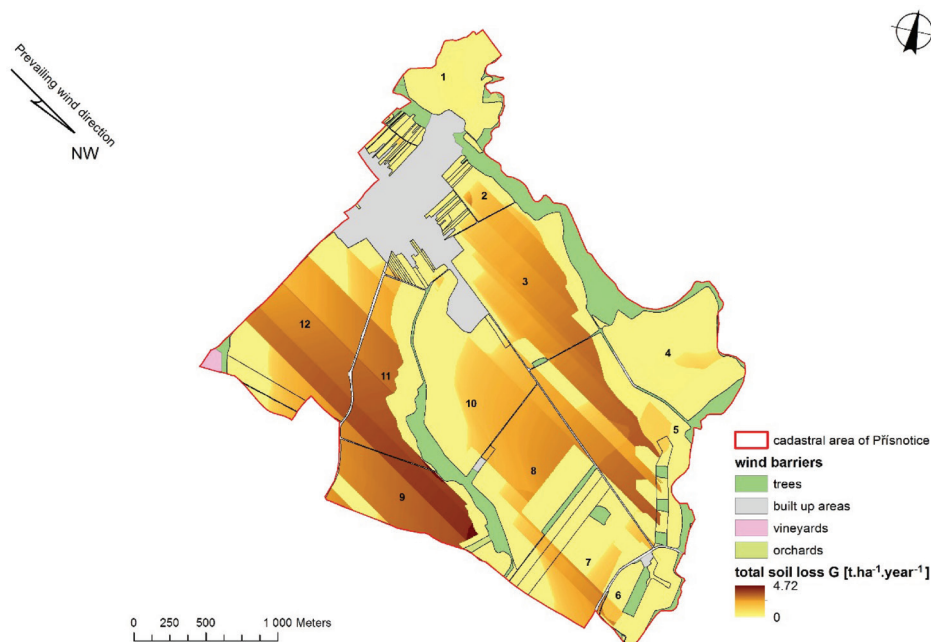
Figure 6. Wind erosion intensity in the cadastral area of Přisnotice in various distances from barriers and protective effect of barriers on their wind – and leeward side
